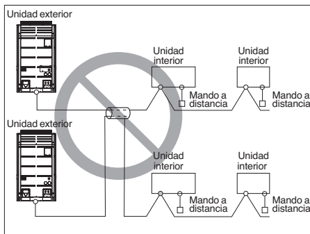
Cable multi-capas
